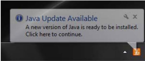
Windows-Auto updates
